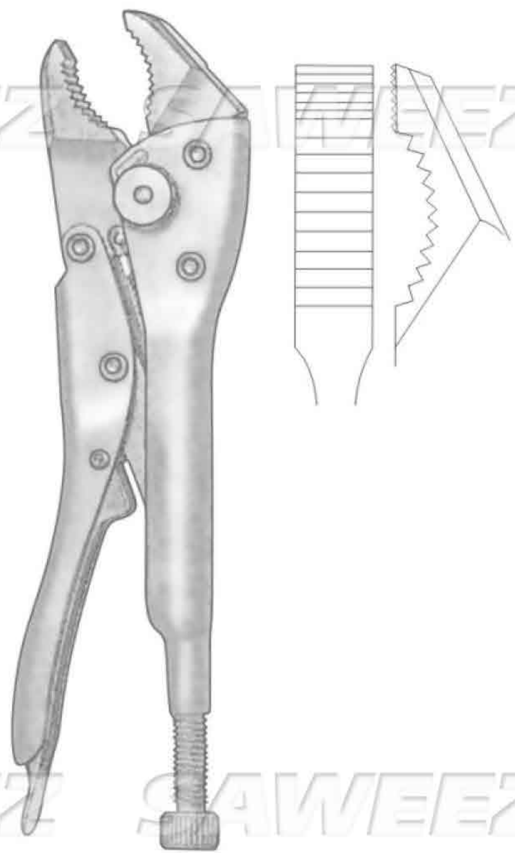
Heavy Duty Locking Pliers SSC-21-11-18 17.0 cm / 6¾" 7mm wide tip reinforced jaw hinge, self-locking lever with adjustment screw and one-handed quick release
