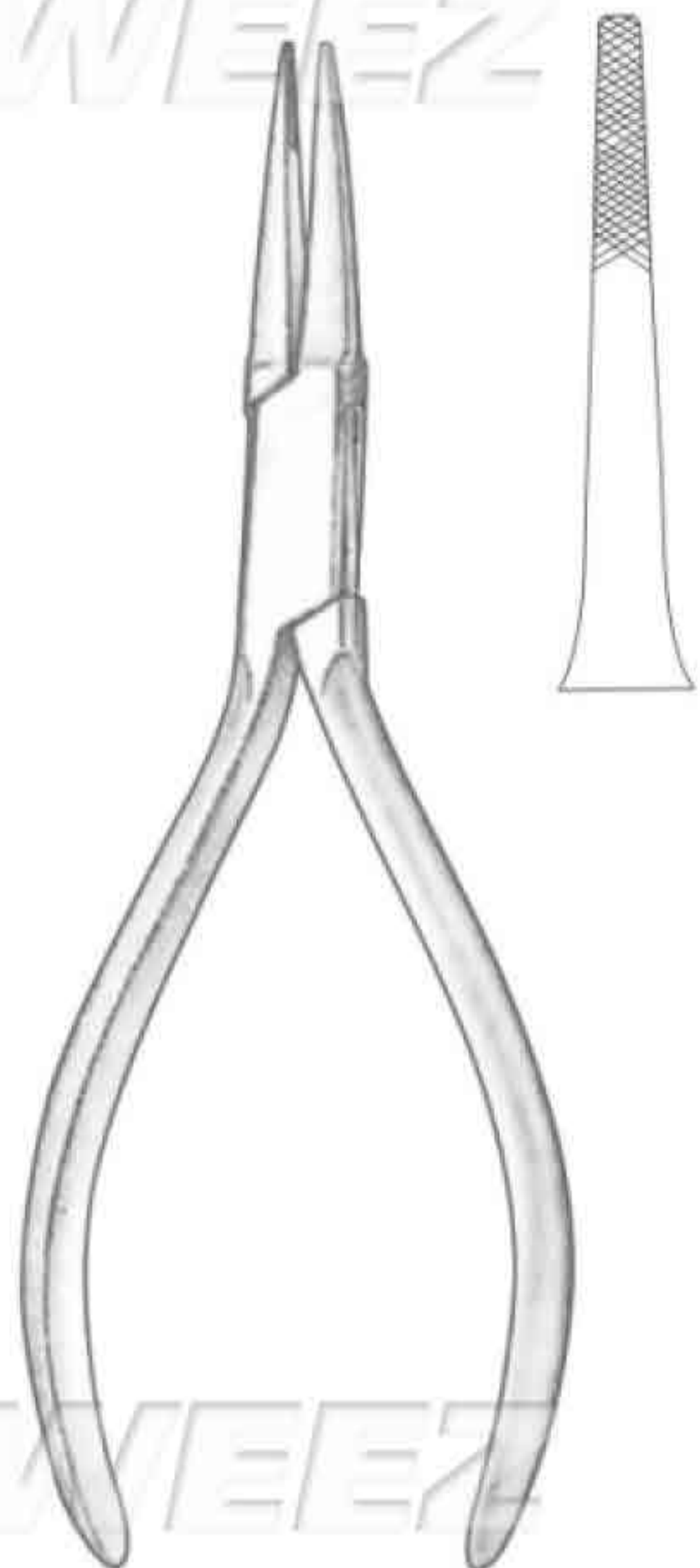
Flat Nose Pliers SSC-21-11-16 15.0 cm / 6", tips taper to 2mm
