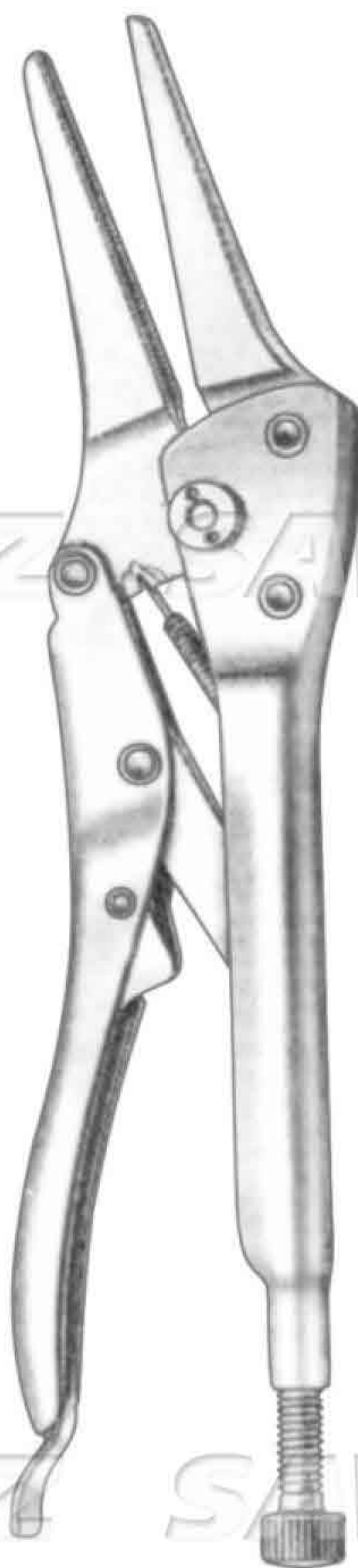
Heavy Duty Locking Pliers SSC-21-11-20 24.0 cm / 9½" 5mm wide tip reinforced jaw hinge, self-locking lever with adjustment screw and one-handed quick release
