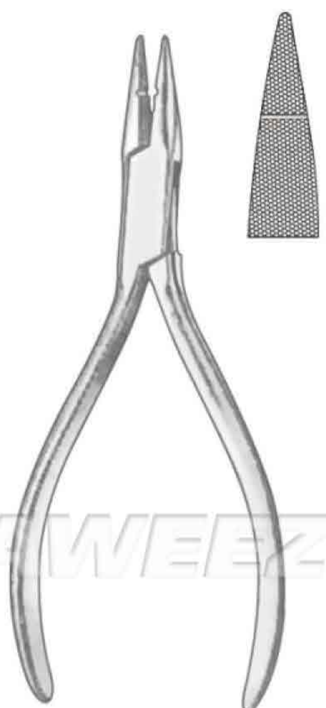
Needle Nose Pliers SSC-21-11-13 14.0 cm / 5½", grooved jaws, tips taper to 1mm
