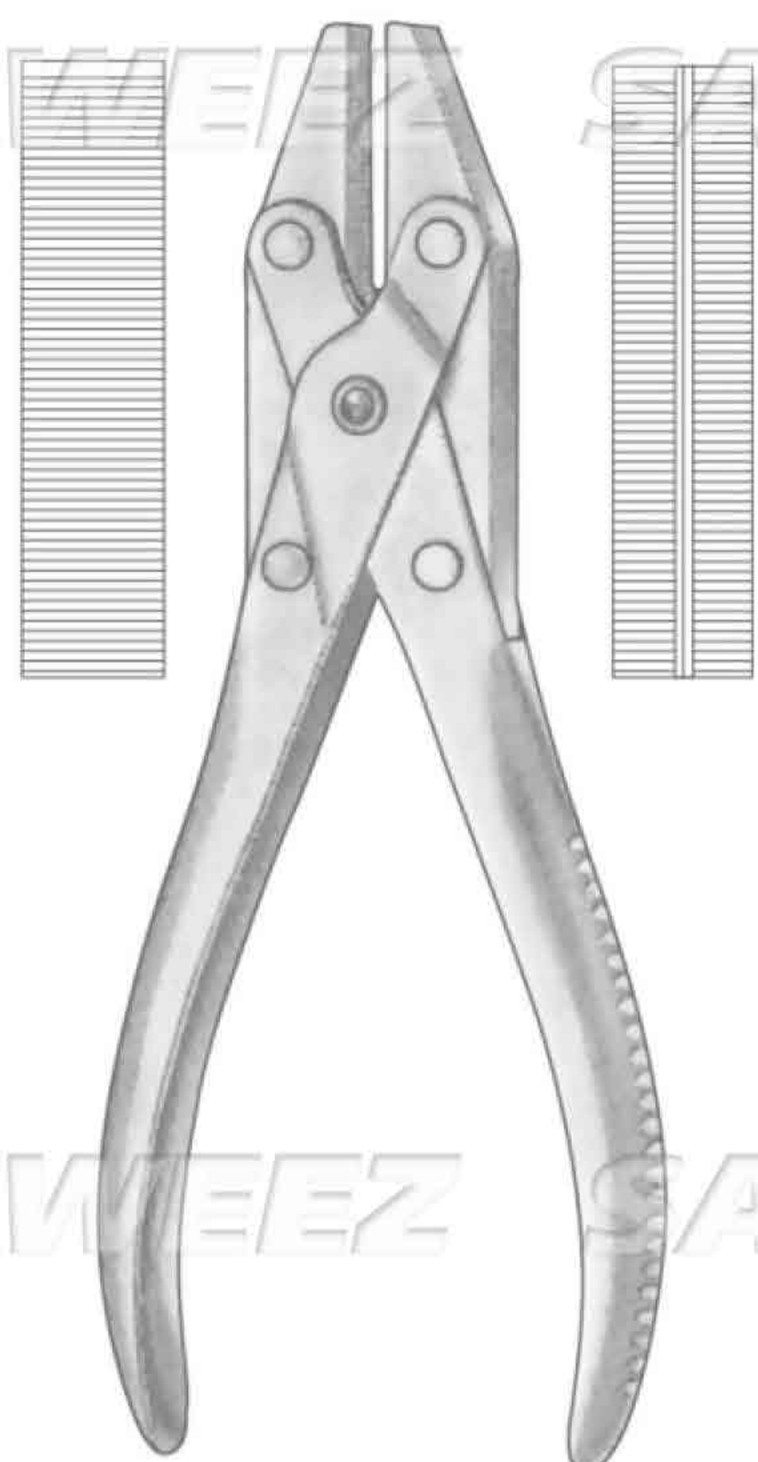
Parallel Pliers SSC-21-11-14 18.0 cm / 7", grooved 10 mm wide jaws for pin removal
