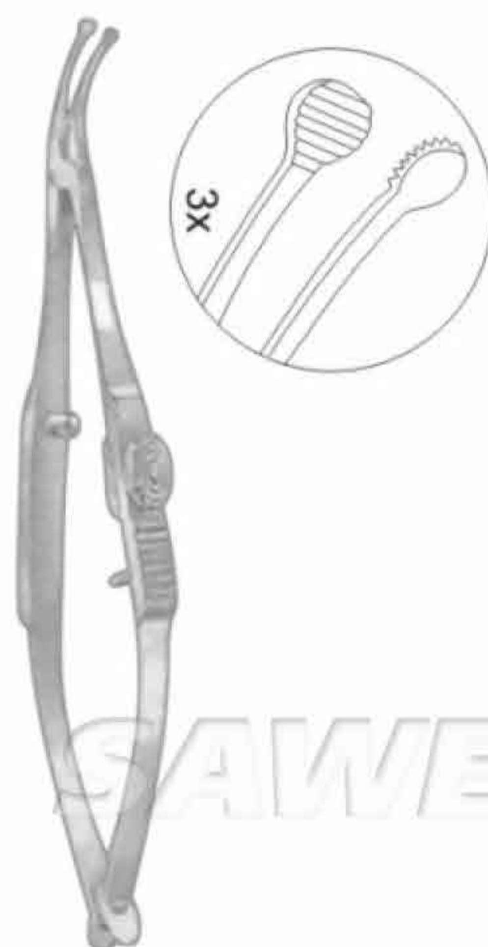
Shepard Intraocular Lens Forceps 9.2 cm / 3 5/8", curved shafts, slide lock, 1.5mm upper and 2mm lower serrated jaws SSC-55-12-05
